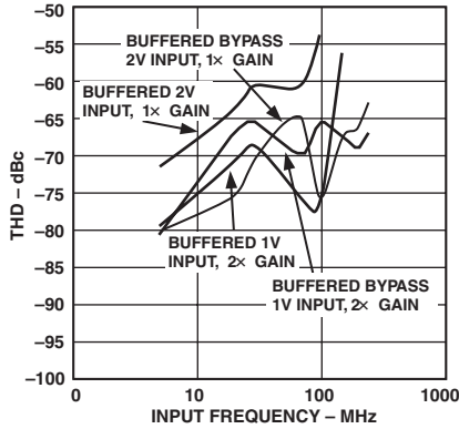
TPC 19. Rx THD vs. f_{IN} , F_{ADC} = 64 \text{ MSPS}
