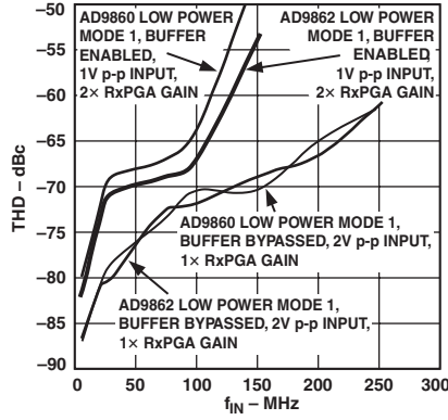
TPC 20. Rx THD vs. f_{IN} , F_{ADC} = 32 \text{ MSPS}
