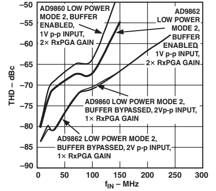
TPC 21. Rx THD vs. f_{IN} , F_{ADC} = 16 \text{ MSPS}
