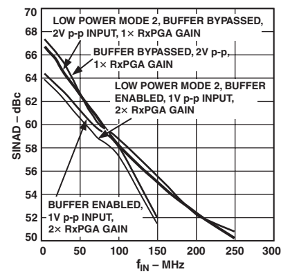
TPC 15. AD9862 Rx SINAD vs. f_{IN} at 16 MSPS
