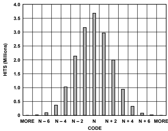
Figure 38. Input Referred Noise Histogram with 2.5 GSPS
