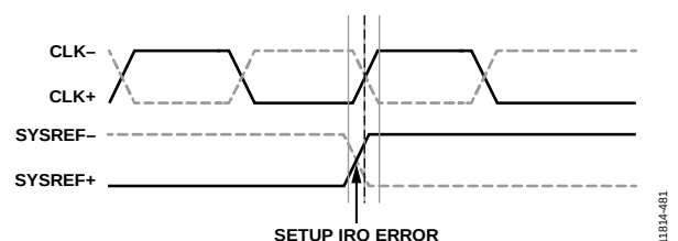
Figure 96. SYSREF± Edge Falls Within the Actual Setup Time Window and Triggers an IRQ Error
