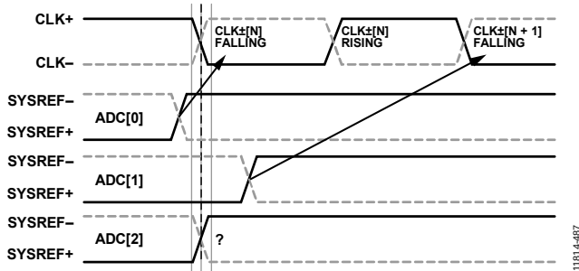
Figure 102. SYSREF± Case From Three ADCs Having Various Phase Delays Relative to the Falling Edge of the Encode Clock and is Latched on Different Sample Clock Edges CLK±[N] or CLK±[N + 1]
