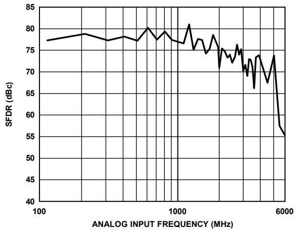
Figure 37. SFDR vs. AIN Frequency at 2.5 GSPS (Input Network in Figure 76 Used <2 GHz, Input Network in Figure 75 used >2 GHz)
