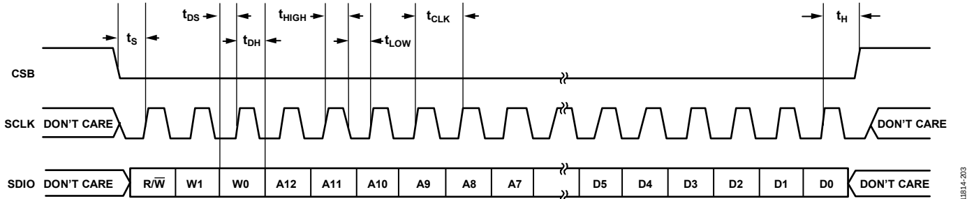
Figure 3. Serial Port Interface Timing Diagram (MSB First)
