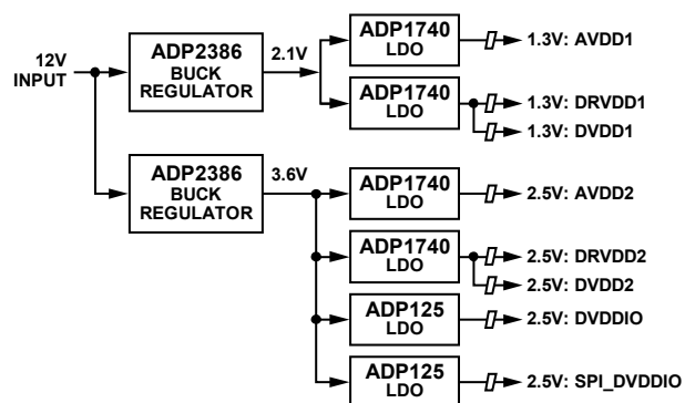
Figure 106. Power Supply Recommendation
