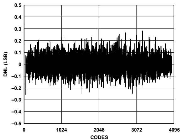
Figure 39. Differential Nonlinearity (DNL), \pm 0.3 LSB at 2.5 GSPS
