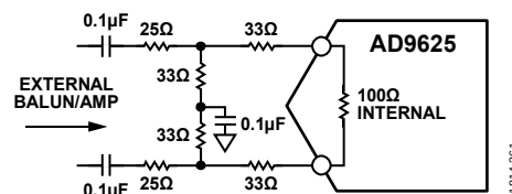
Figure 76. Input Network Example for Passive Balun and <2 GHz ADC Bandwidth
