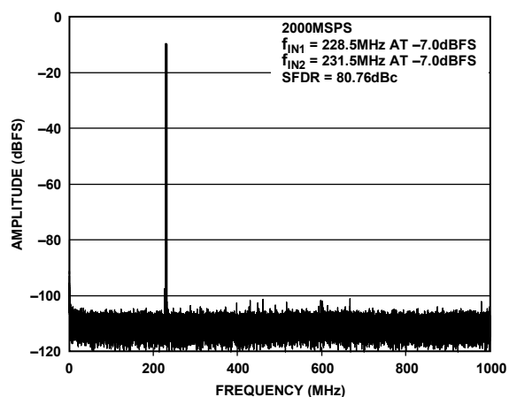
Figure 22. Two Tone FFT Plot at 2.0 GSPS, f_{IN1} = 228.5 MHz and f_{IN2} = 231.5 MHz at AIN, -7.0 dBFS (SFDR = 80.76 dBc)
