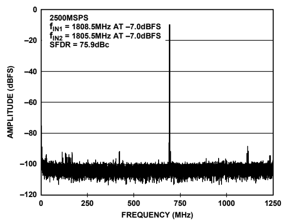
Figure 41. Two Tone FFT Plot at 2.5 GSPS, f_{IN1} = 1808.5 MHz and f_{IN2} = 1805.5 MHz at AIN, -7.0 dBFS (SFDR = 75.9 dBc)
