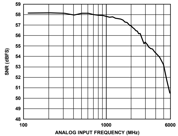
Figure 40. SNR vs. AIN Frequency at 2.5 GSPS (Input Network in Figure 76 Used <2 GHz, Input Network in Figure 75 Used >2 GHz)
