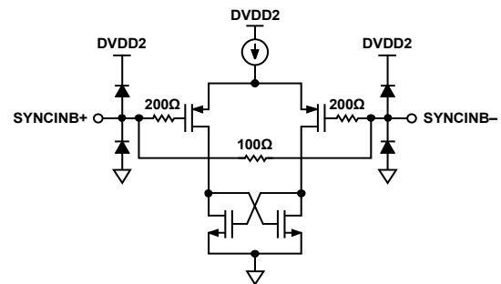
Figure 68. Equivalent SYNCINB± Input
