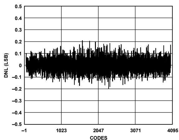
Figure 23. Differential Nonlinearity (DNL), \pm 0.2 LSB at 2.0 GSPS
