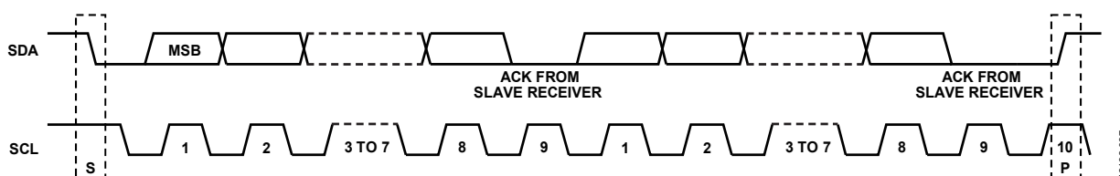
Figure 45. Acknowledge Bit
