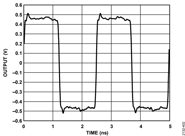
Figure 16. Output Waveform, 14 mA LVDS-Compatible Mode (400 MHz) with 100 \Omega Termination at Load
