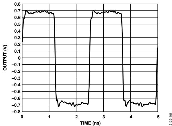
Figure 15. Output Waveform, 21 mA Mode (400 MHz) with 100 \Omega Termination at Load
