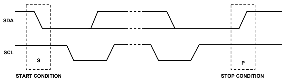
Figure 44. Start and Stop Conditions
