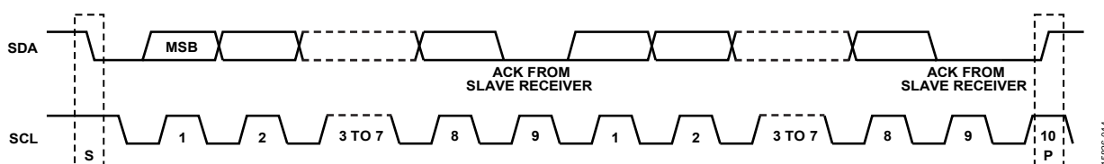
Figure 61. Acknowledge Bit
