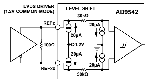
Figure 28. Differential LVDS Input Mode
