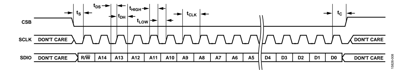
Figure 55. Timing Diagram for Serial Control Port Write—MSB First
