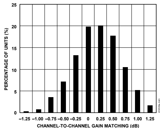
Figure 10. Gain Match Histogram, GAIN+ = 1.3 V
