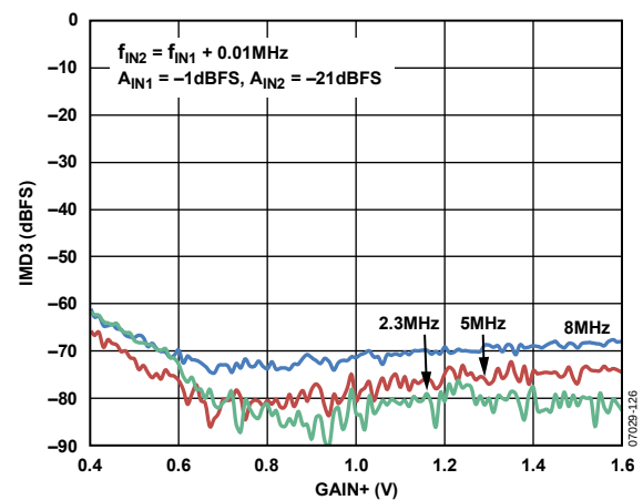
Figure 22. IMD3 vs. GAIN+
