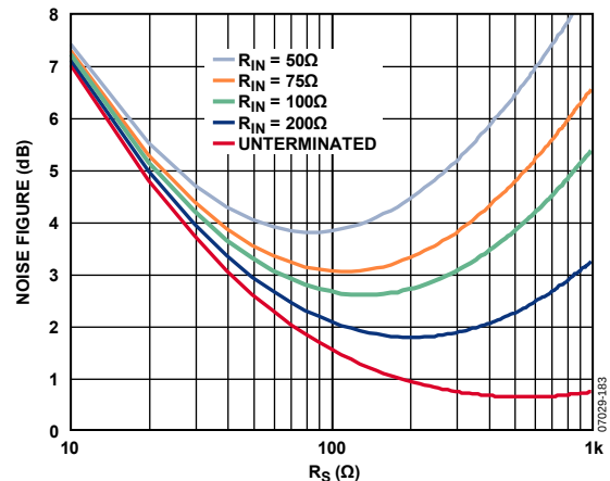
Figure 42. Noise Figure vs. R_S for Various Fixed Values of R_{IN} , Active Termination Matched Inputs, V_{\text{GAIN}} = 0.8 \text{ V}
