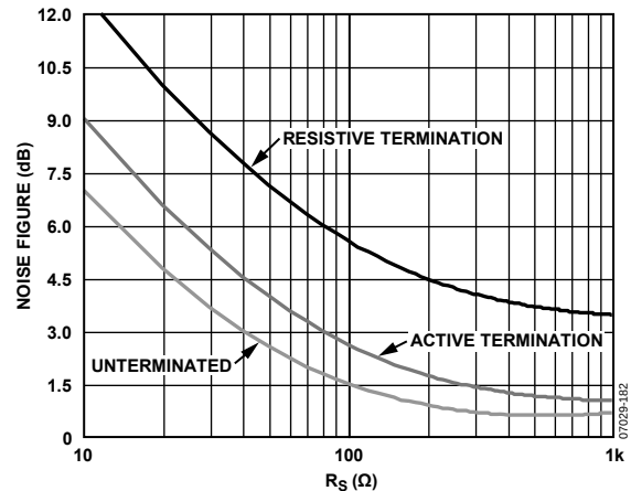
Figure 41. Noise Figure vs. R_S for Resistive Termination, Active Termination Matched, and Untermi-nated Inputs, V_{\text{GAIN}} = 0.8 \text{ V}
