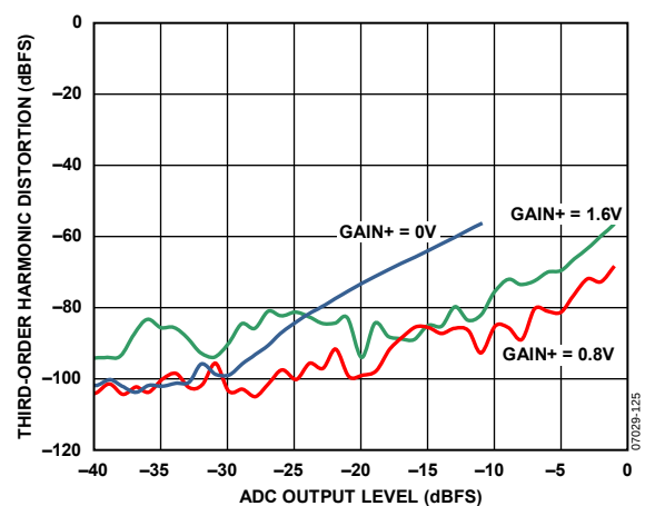
Figure 21. Third-Order Harmonic Distortion vs. ADC Output Level
