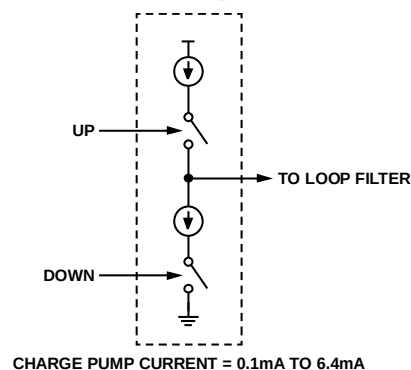
Figure 77. Charge Pump
