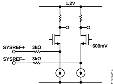
Figure 50. SYSREF± Input Circuit
