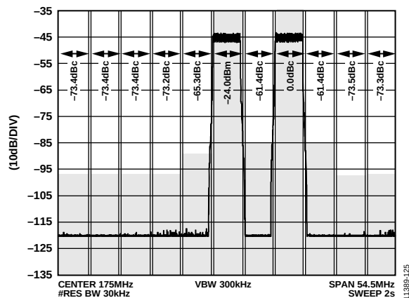
Figure 25. 2-Channel (2C) 5 MHz BW with 5 MHz Gap, LTE ACLR Performance, IF = 180 MHz, f_{DAC} = 1966.08 MHz (Total LTE Carrier Power is 20.982 dBm)
