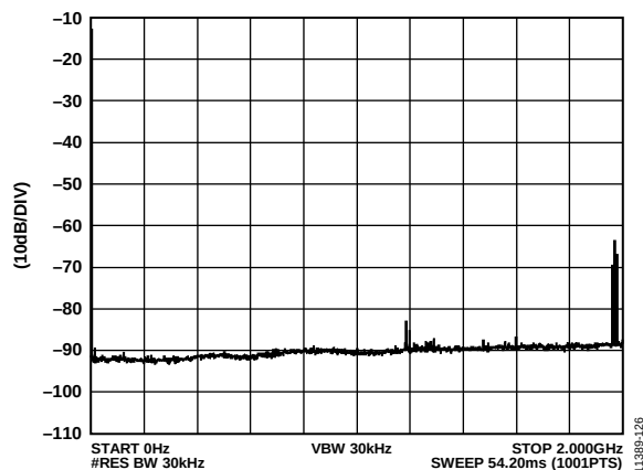
Figure 26. Single Tone SFDR f_{DAC} = 1966.08 MHz, 4x Interpolation, f_{OUT} = 10 MHz, -14 dBFS
