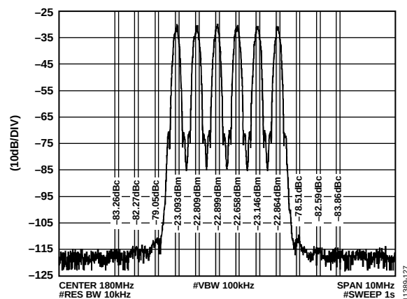
Figure 27. 6-Channel (6C) Spaced by 600 kHz GSM, Enhanced Data Rates for GSM Evolution (EDGE) Adjacent Channel Power (ACP) IMD Performance, IF = 180 MHz, f_{DAC} = 1966.08 MHz
