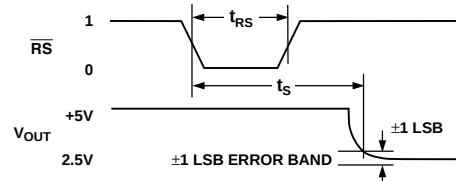
RESET TIMING
