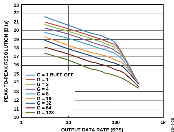
Figure 55. Peak-to-Peak Resolution vs. Output Data Rate (Settled), \text{Sinc}^3 + \text{Sinc}^1 Filter (Mid Power Mode)
