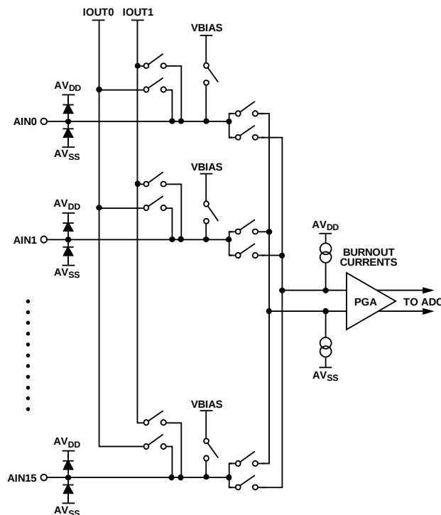
Figure 80. Excitation Current and Bias Voltage Connections
