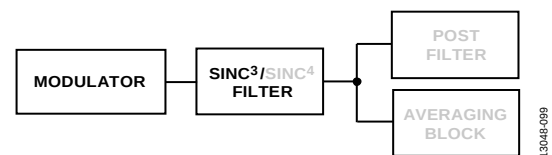
Figure 92. Sinc 3 Filter
