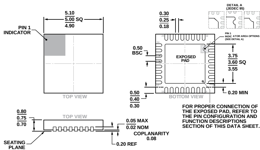
Figure 132. 32-Lead Lead Frame Chip Scale Package [LFCSP] 5 mm x 5 mm Body and 0.75 mm Package Height (CP-32-12)
