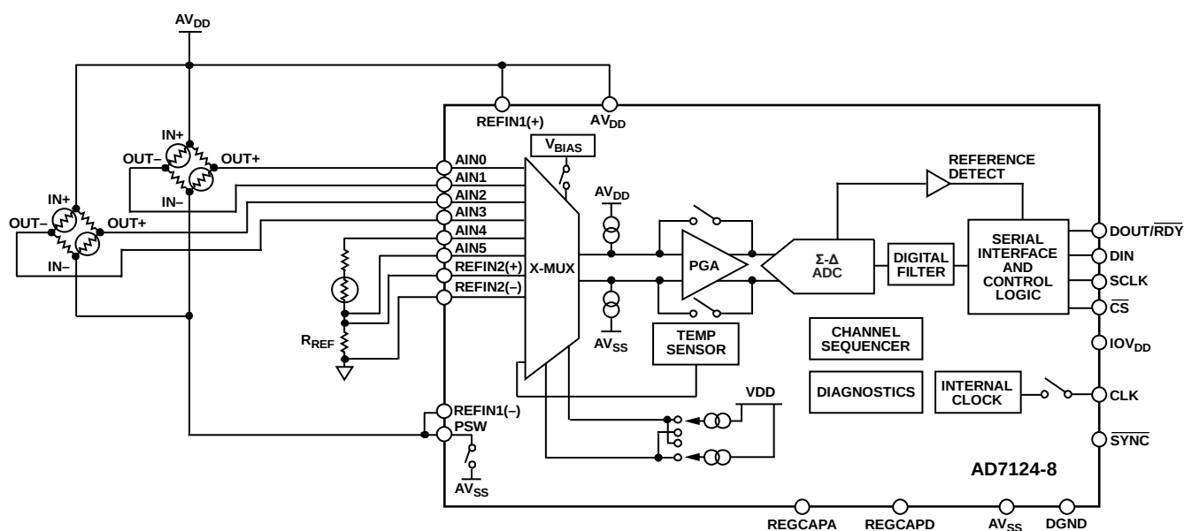
Figure 131. Flowmeter Application
