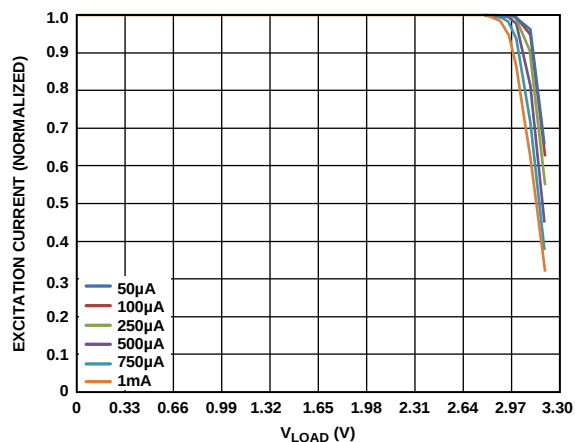
Figure 34. Output Compliance ( AV_{DD} = 3.3\text{ V} )
