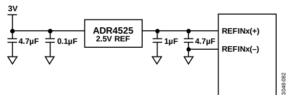
Figure 79. ADR4525 to AD7124-8 Connections
