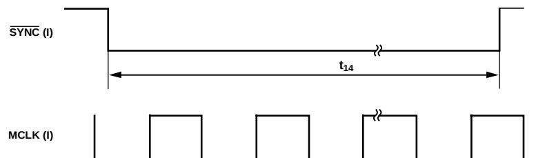
Figure 8. \overline{SYNC} Pulse Width
