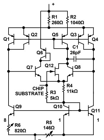
Figure 7. Schematic Diagram
