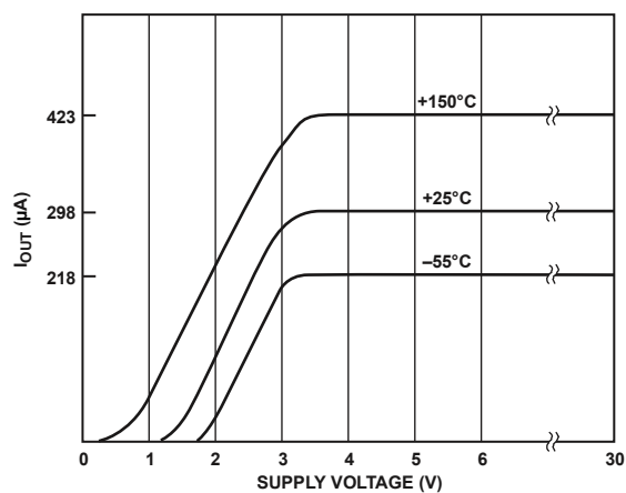
Figure 8. V-I Plot
