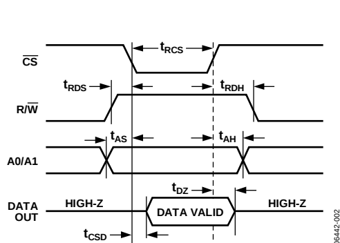
Figure 2. Data Read Timing
