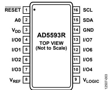
Figure 3. 16-Lead TSSOP Pin Configuration
