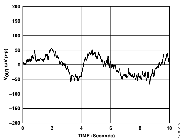
Figure 23. DAC 1/f Noise with External Reference
