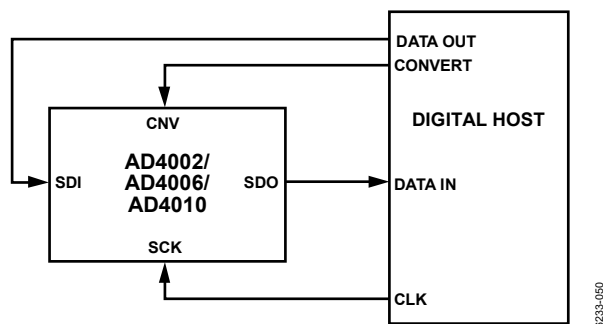
Figure 51. \overline{CS} Mode, 3-Wire Turbo Mode Connection Diagram
