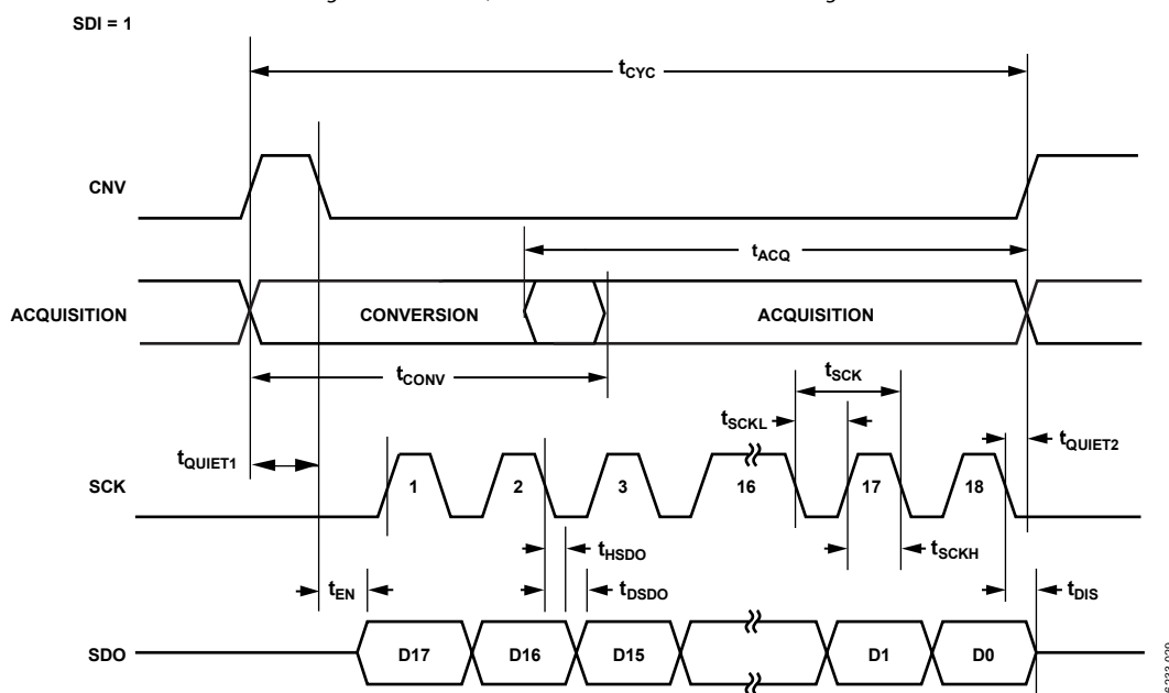
Figure 52. \overline{\text{CS}} Mode, 3-Wire Turbo Mode Serial Interface Timing Diagram (Status Bits Not Shown)
