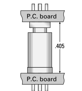
Straight P.C. board plug (7225 series) and straight P.C. board jack (7209 series)
