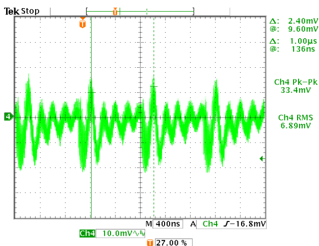
Figure 48. Input Voltage Noise with Interleave
