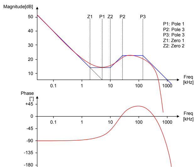
Figure 52. Transfer Function of PWM
