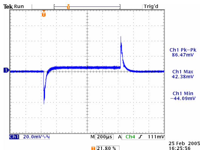
Figure 17. Vin=5V, Vout=1V, BW=40kHz
