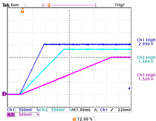
Figure 9. Turn-On with Different Rising Slew Rates. Rising Slew Rates are Programmed as follows: V1- 1V/ms, V2-0.5V/ms, V3-0.2V/ms. V_{in}=12V , Ch1 – V1, Ch2 – V2, Ch3 – V3
