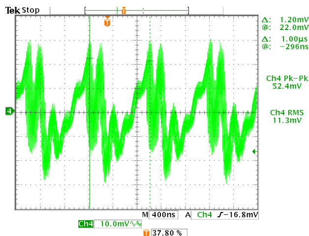
Figure 47. Input Voltage Noise, No Interleave
