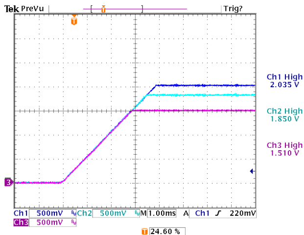
Figure 8. Tracking Turn-On. Rising Slew Rate is Programmed at 0.5V/ms. V_{in}=12V , Ch1 – V1, Ch2 – V2, Ch3 – V3
