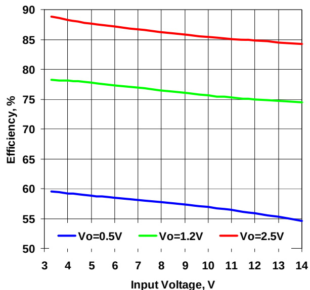
Figure 7. Efficiency vs. Input Voltage. I_{out}=7A , F_{sw}=500kHz
