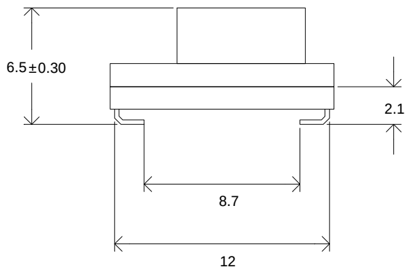
Figure 57. Side View
