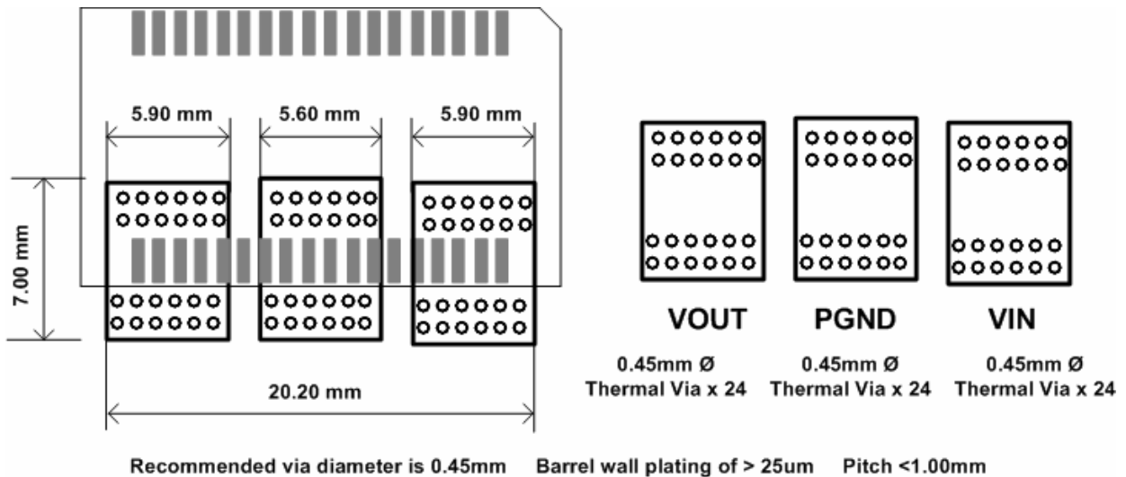
Figure 60. Recommended PCB Layout for Multilayer PCBs
