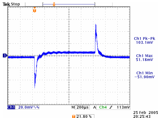
Figure 16. Vin=5V, Vout=2.5V, BW=40kHz
