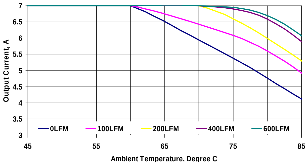
Figure 19. Thermal Derating Curves. V_{in}=12V , V_{out}=5.0V , F_{sw}=500kHz
