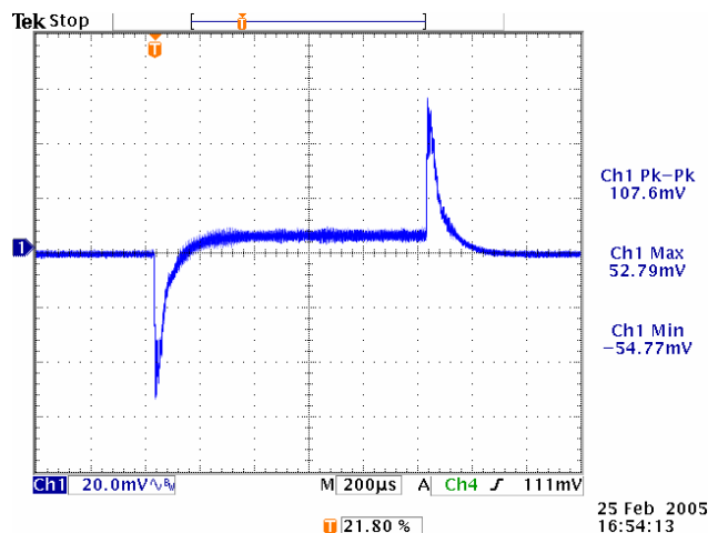
Figure 18. Vin=3.3V, Vout=1V, BW=40kHz
