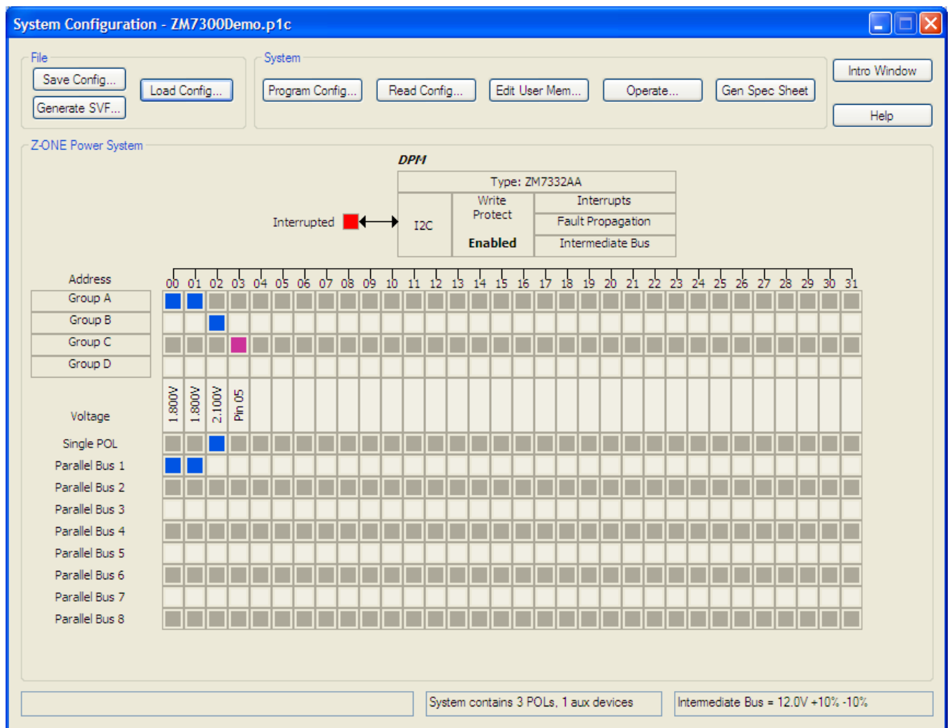
Figure 53. GUI System Configuration Window
