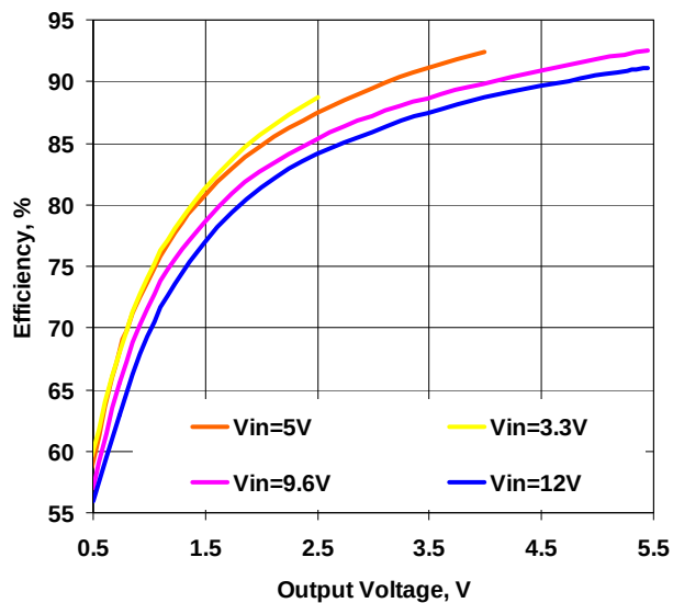
Figure 6. Efficiency vs. Output Voltage, I_{out}=7A , F_{sw}=500kHz
