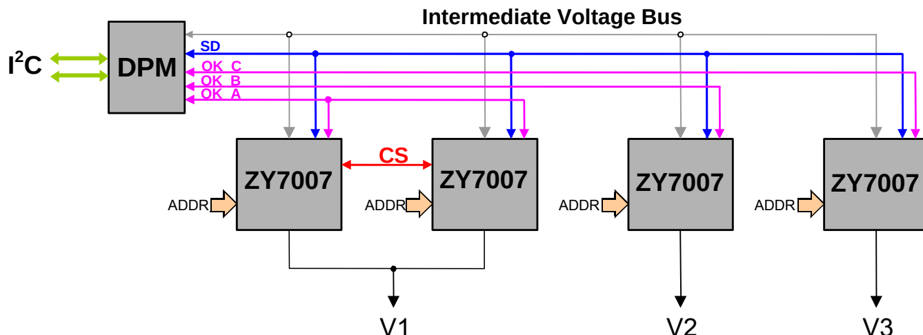
Figure 23. Block Diagram of Typical Multiple Output Application with Digital Power Manager and I²C Interface
