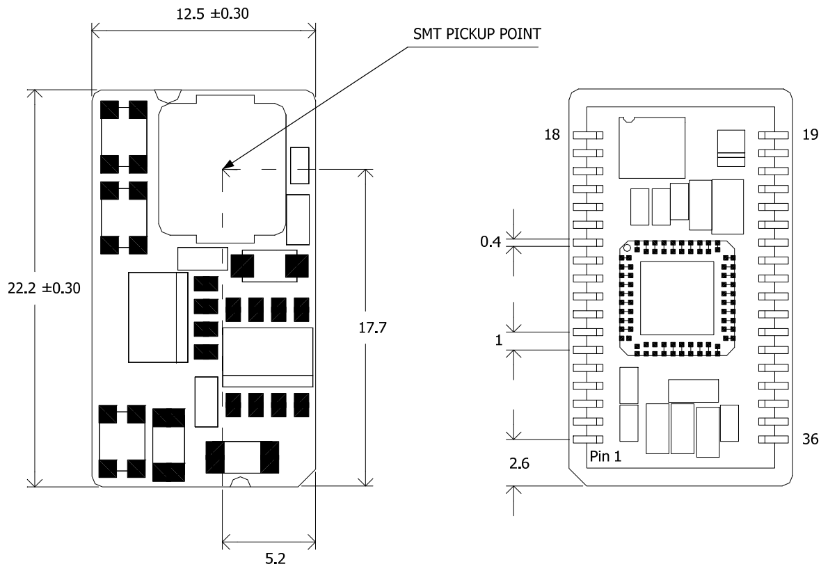
Figure 56. Top (Left) and Bottom Views
