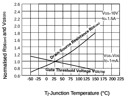
Normalized R_{DS(on)} and V_{GS(th)} v Temperature
