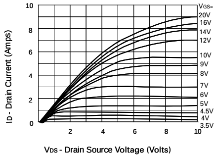
Saturation Characteristics
