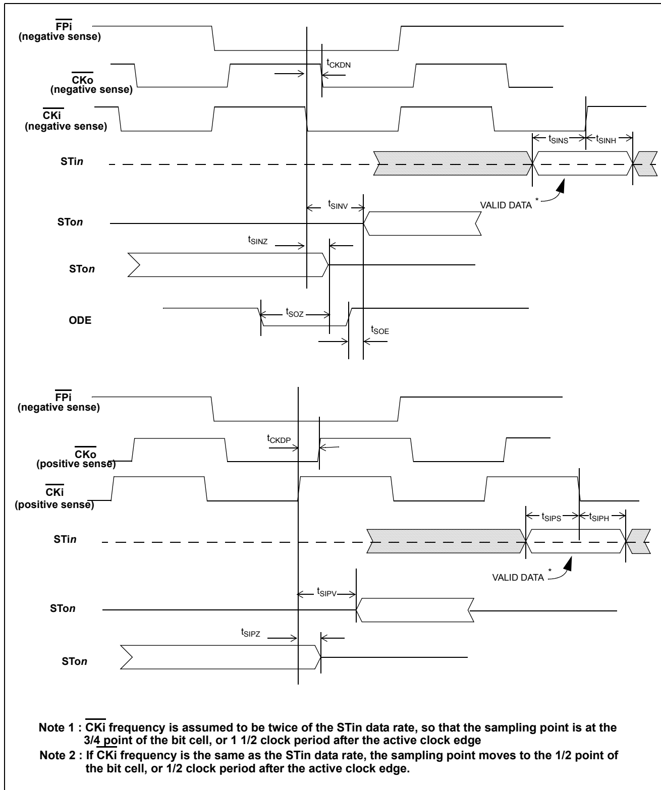
Figure 14 - Serial Data Timing to CKi
