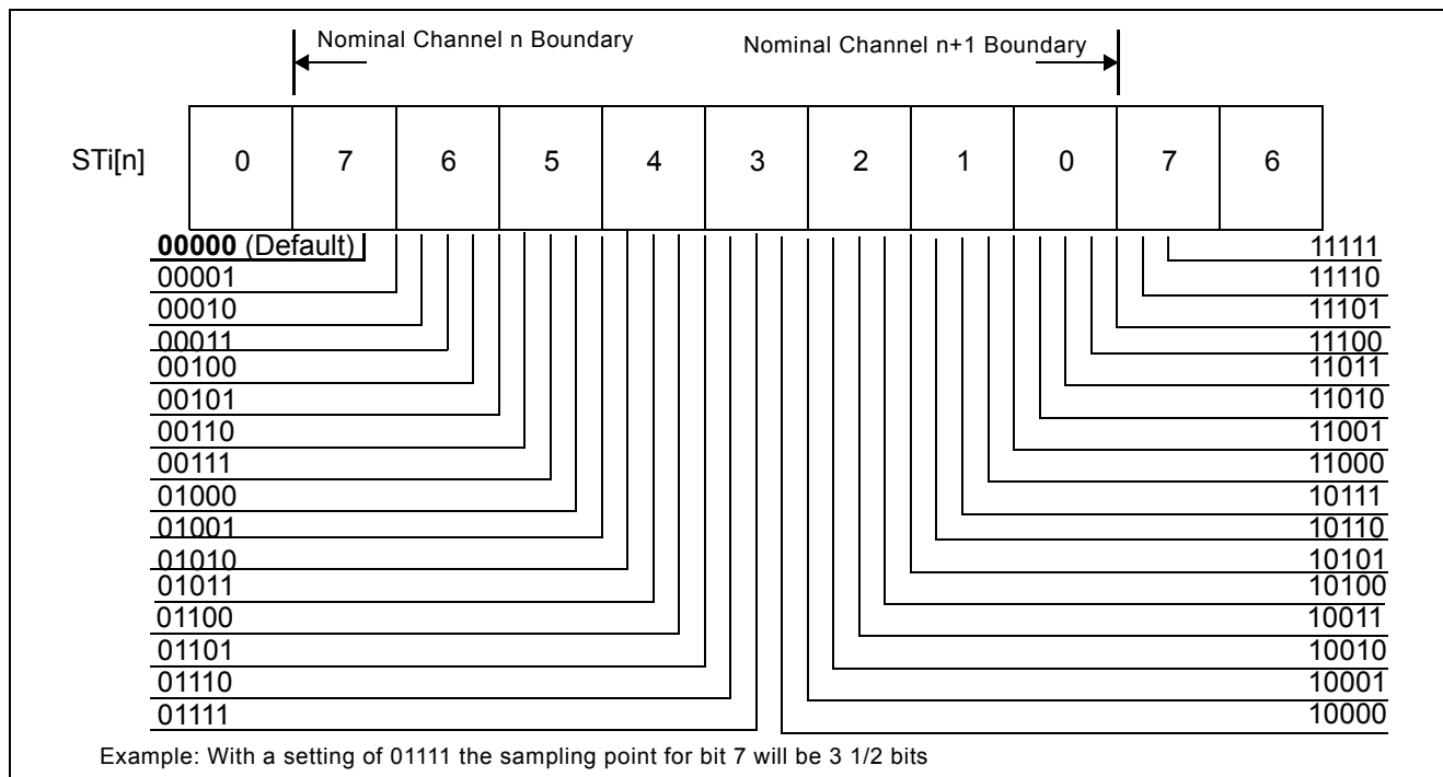
Figure 4 - Input Sampling Point Delay Programming
