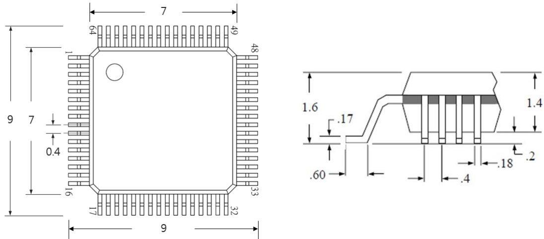
Figure 12. Package Dimension Information
