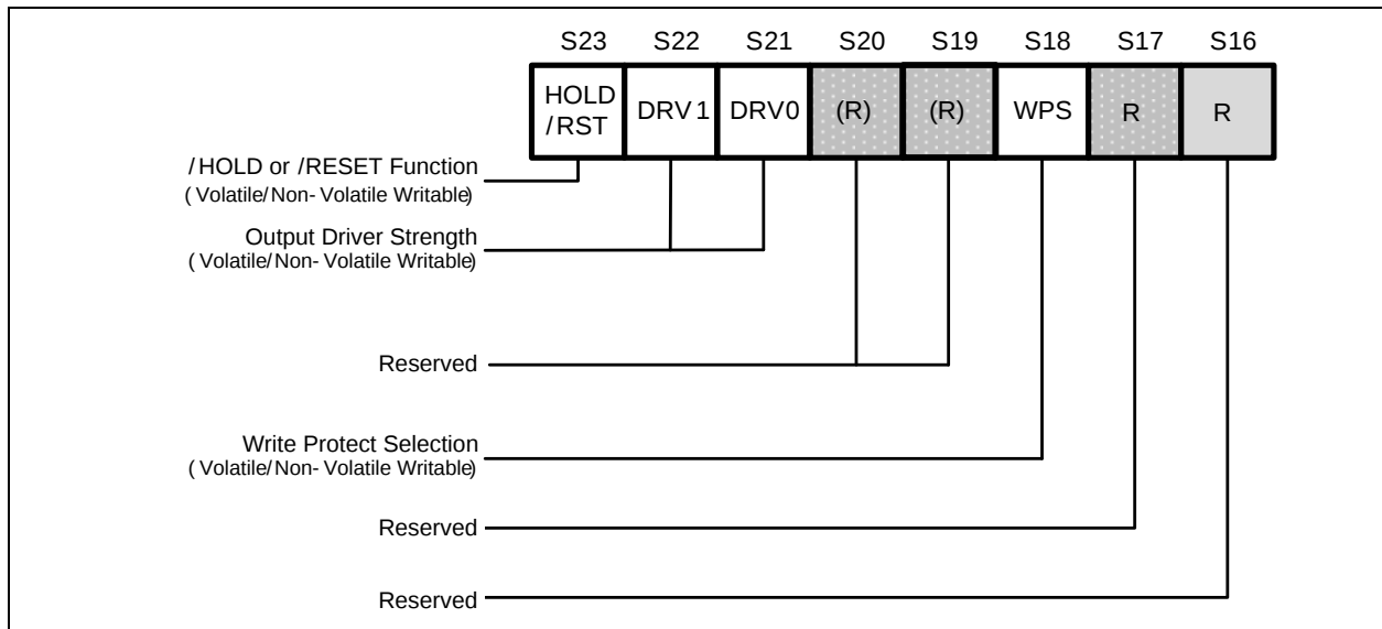
Figure 4c. Status Register-3
