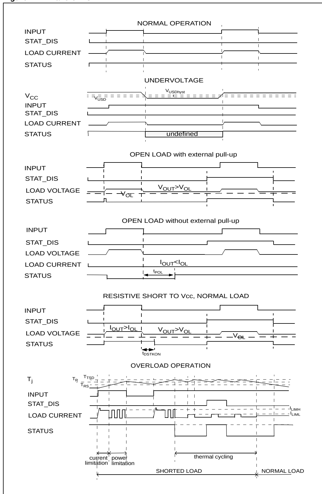
Figure 7. Waveforms
