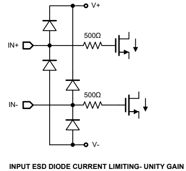
INPUT ESD DIODE CURRENT LIMITING- UNITY GAIN
