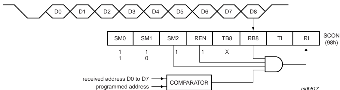
UART modes 2 or 3 and SM2 = 1: there is an interrupt if REN = 1, RB8 = 1 and received address is equal to programmed address. When own address is received, reset SM2 to receive the data bytes. When all data bytes are received, set SM2 to wait for the next address.
