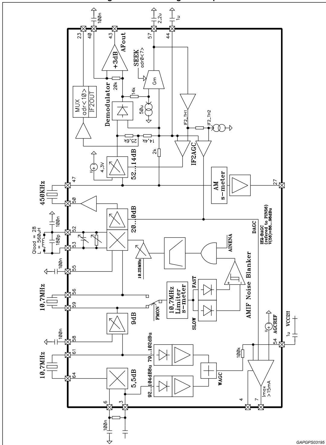
Figure 13. Block diagram AM path
