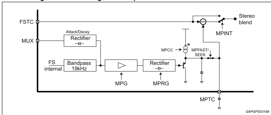
Figure 16. Block diagram multi path detection for stereo decoder
