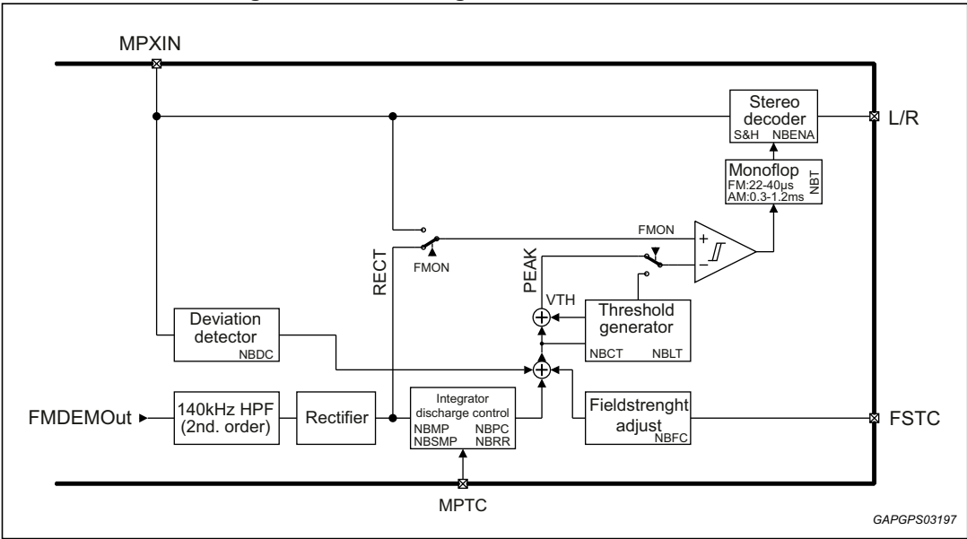
Figure 15. Block diagram audio noise blanker
