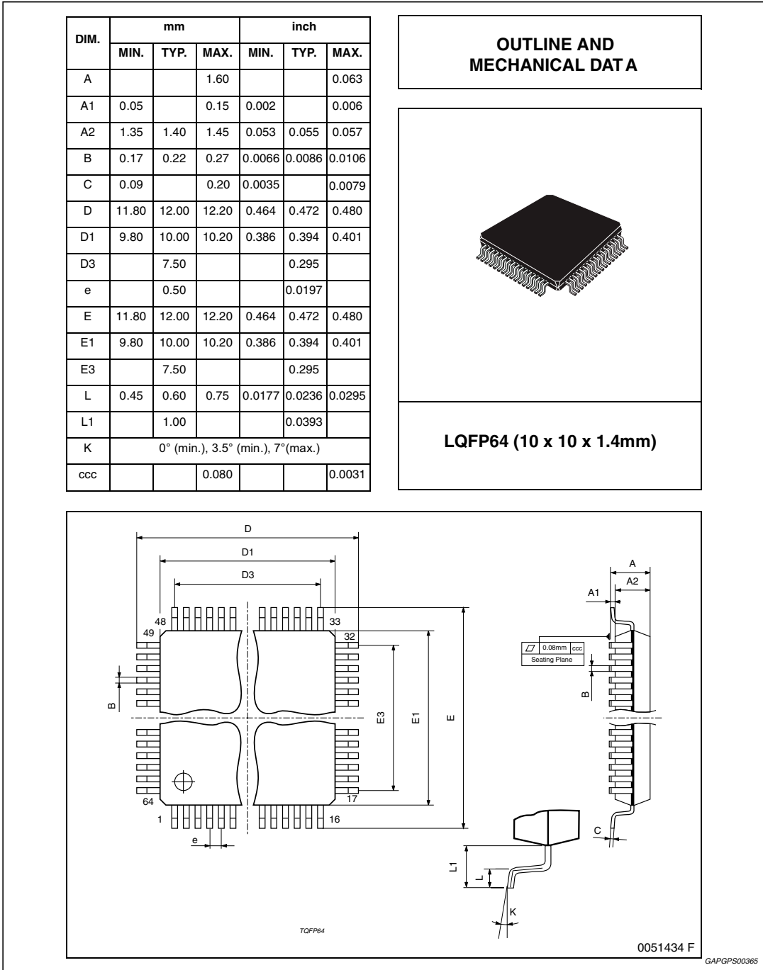
Figure 8. LQFP64 (10x10x1.4 mm) mechanical data and package dimensions
