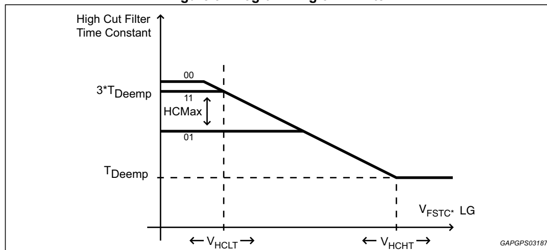
Figure 3. Programming of HC filter
