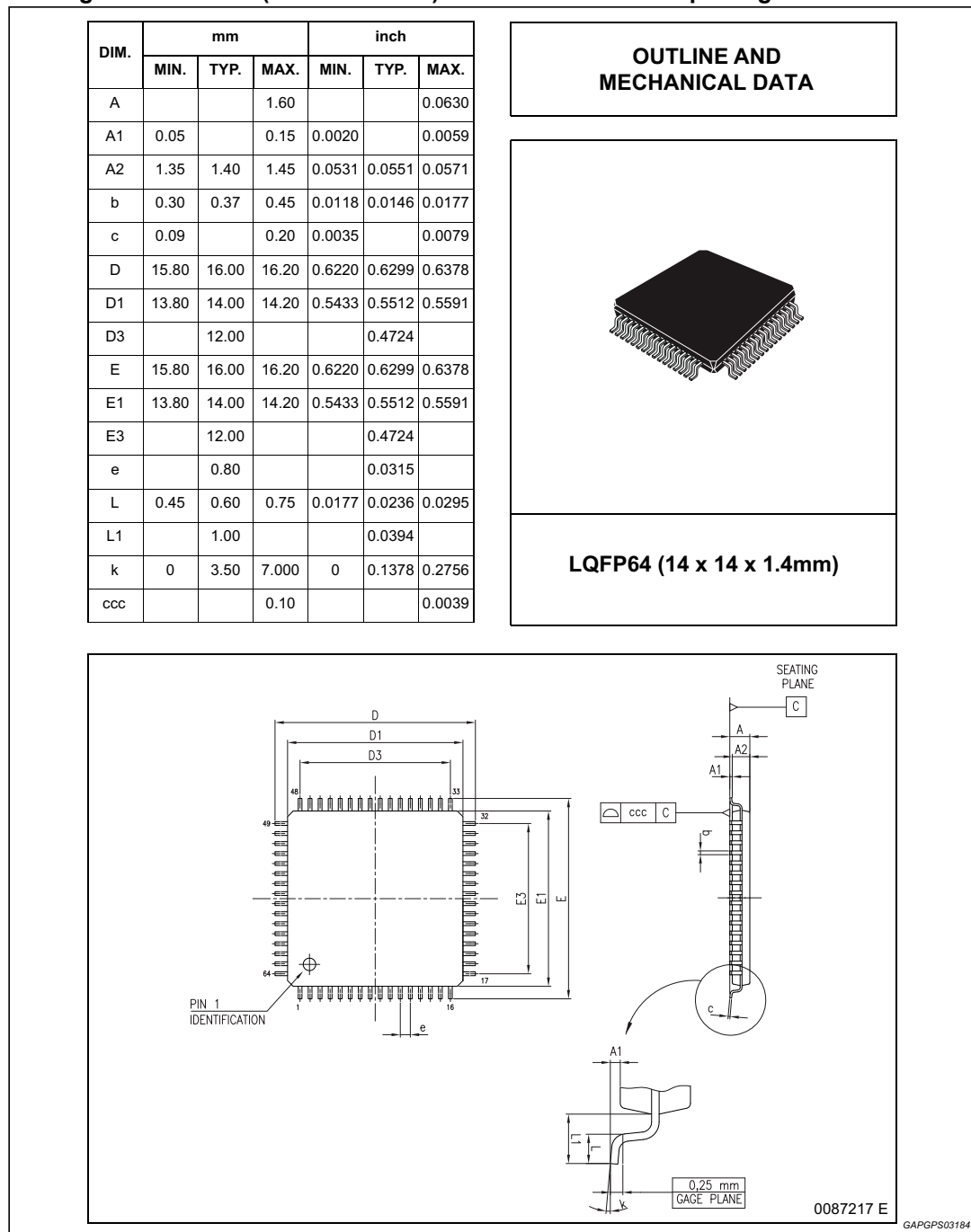
Figure 9. LQFP64 (14x14x1.4 mm) mechanical data and package dimensions
