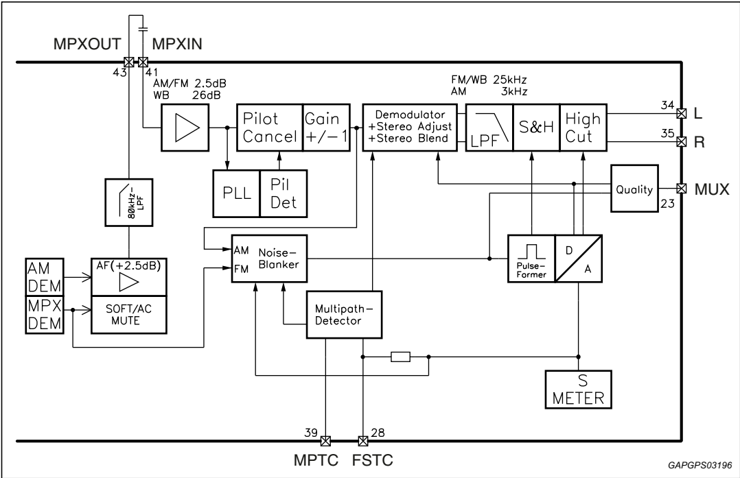
Figure 14. Block diagram stereo decoder
