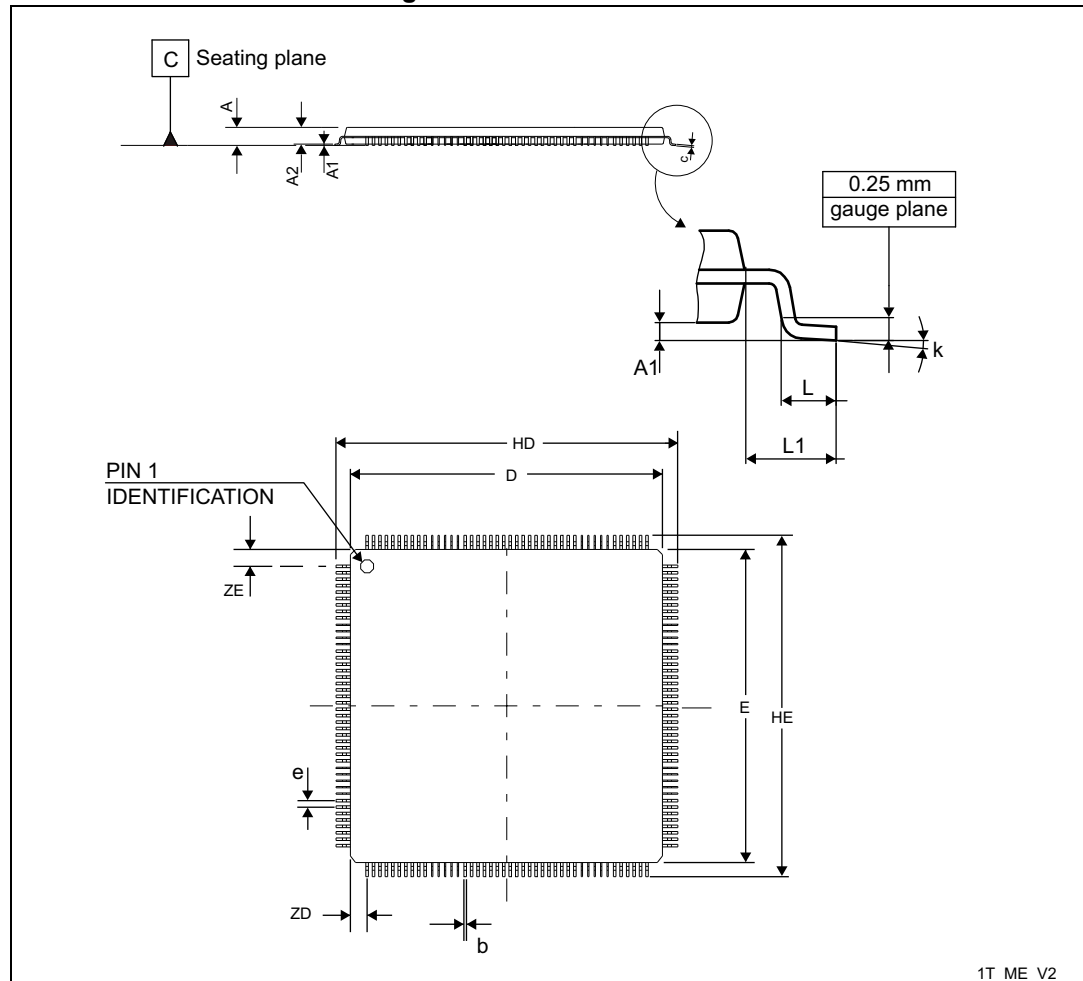
Figure 92. LQFP176 outline
