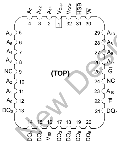
Figure 2. Pin Diagram - 32-Pin 450 Mil LCC
