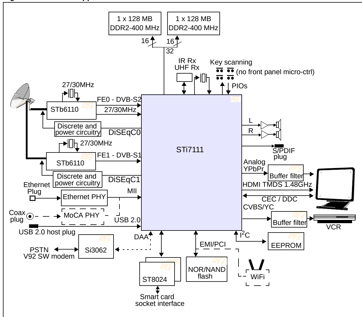
Figure 1. STi7111 applications
