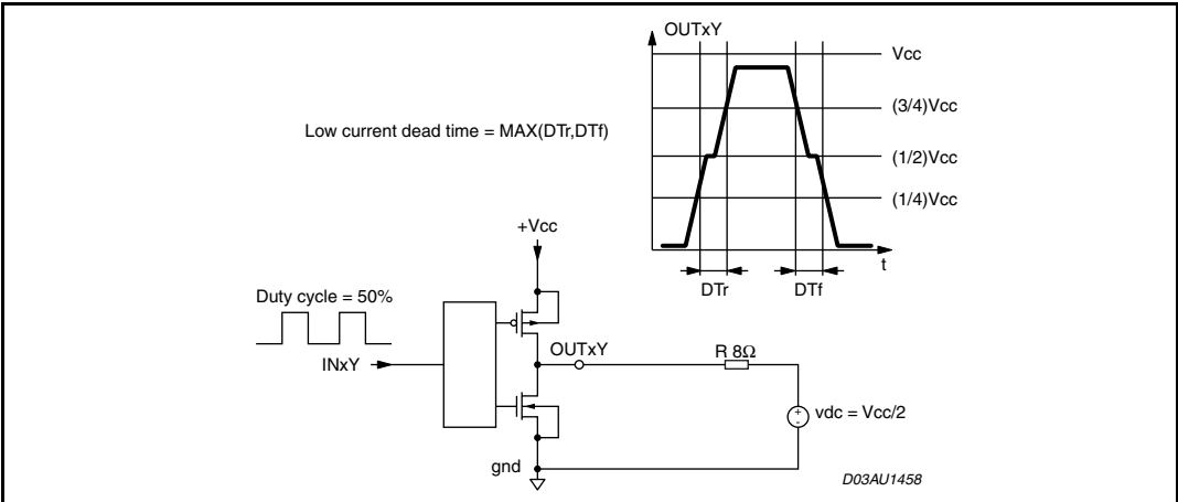
Figure 3. Test circuit
