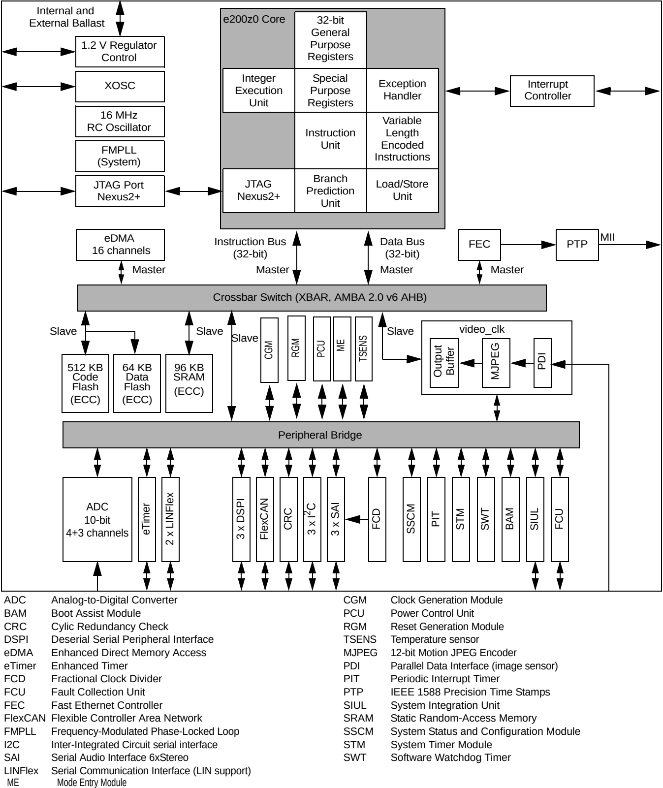
Figure 1. MPC5604E block diagram
