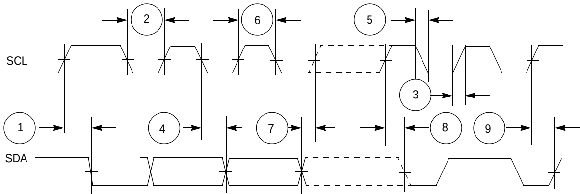
Figure 36. I²C input/output timing
