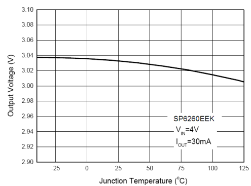
Fig. 14: Output Voltage vs. Junction Temperature SP6260EEK-L (3.0V)
