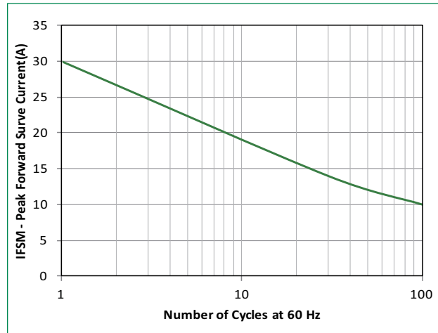
Figure 8 - Maximum Non-Repetitive Forward Surge Current Uni-Directional Only
