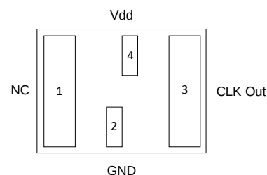
Figure 1. Pin Assignments
