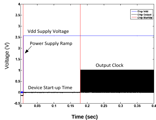
Figure 11. Start-up Time
