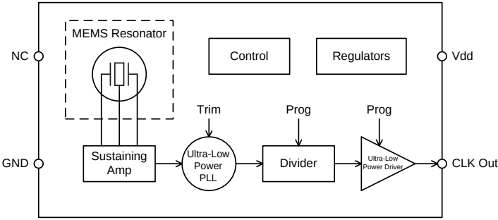
Figure 2. SiT1533 Block Diagram
