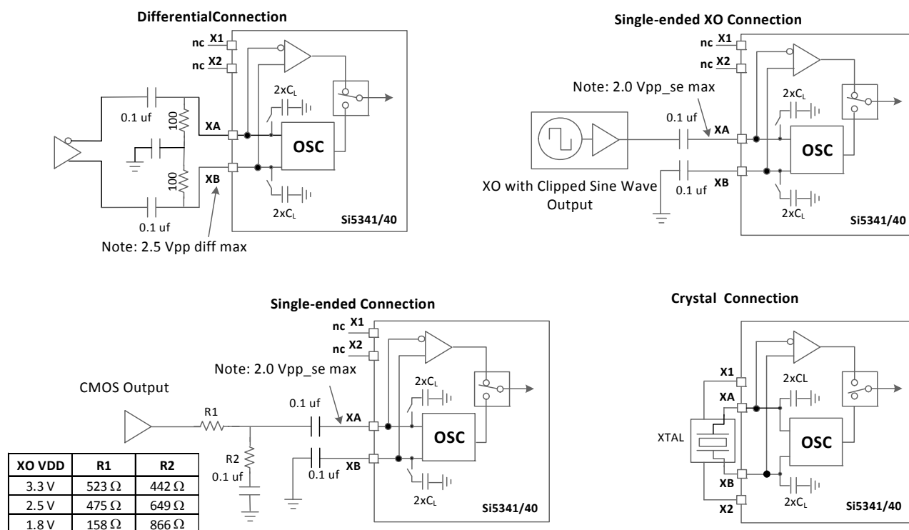
Figure 11. XAXB External Crystal and Clock Connections
