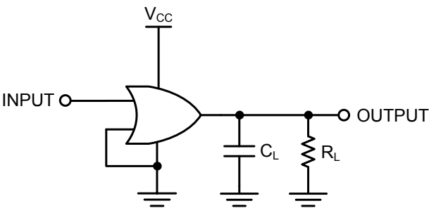
CL includes load and stray capacitance; Input PRR = 10MHz; t_W = 500\text{ns} .
