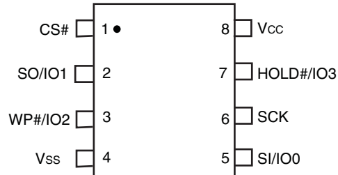
Figure 27. 8-Pin Plastic Small Outline Package (SO)
