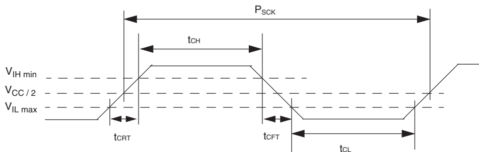
Figure 20. Clock Timing
