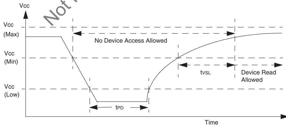
Figure 19. Power-Down and Voltage Drop
