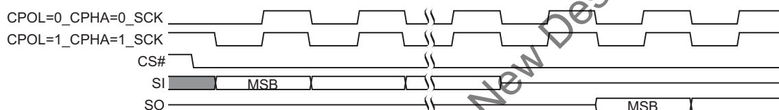
Figure 4. SPI Modes Supported
