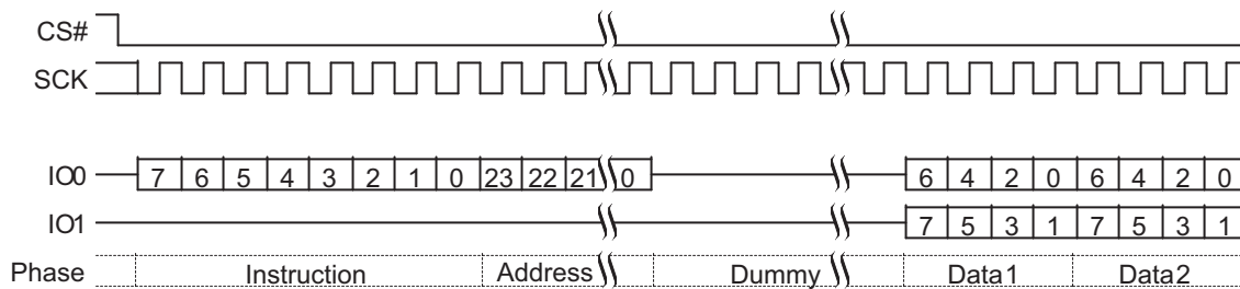
Figure 10. Dual Output Command
