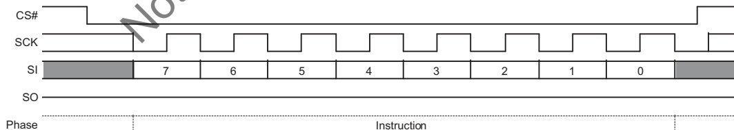
Figure 33. Write Enable for Volatile Status Register Command Sequence
