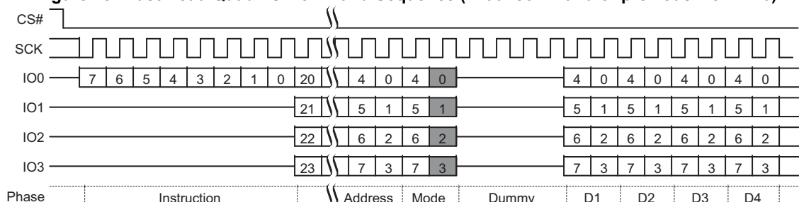
Figure 48. Fast Read Quad I/O Command Sequence (Initial command or previous M5-4 ≠ 10)
