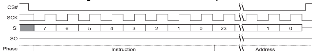
Figure 37. Sector Erase Command Sequence
