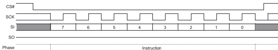
Figure 39. Chip Erase Command Sequence
