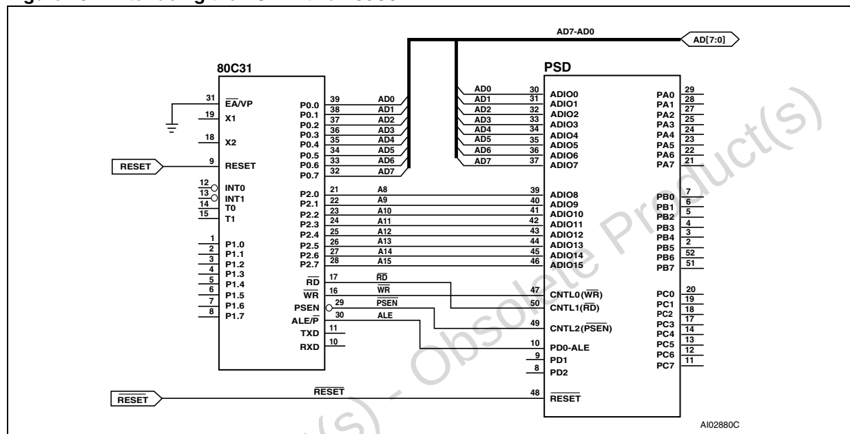
Figure 20 shows the bus interface for the 80C31, which has an 8-bit multiplexed address/data bus. The lower address byte is multiplexed with the data bus. The MCU control signals Program Select Enable ( \overline{\text{PSEN}} , CNTL2), Read Strobe ( \overline{\text{RD}} , CNTL1), and Write Strobe ( \overline{\text{WR}} , CNTL0) may be used for accessing the internal memory and I/O ports blocks. Address Strobe (ALE/AS, PD0) latches the address.
