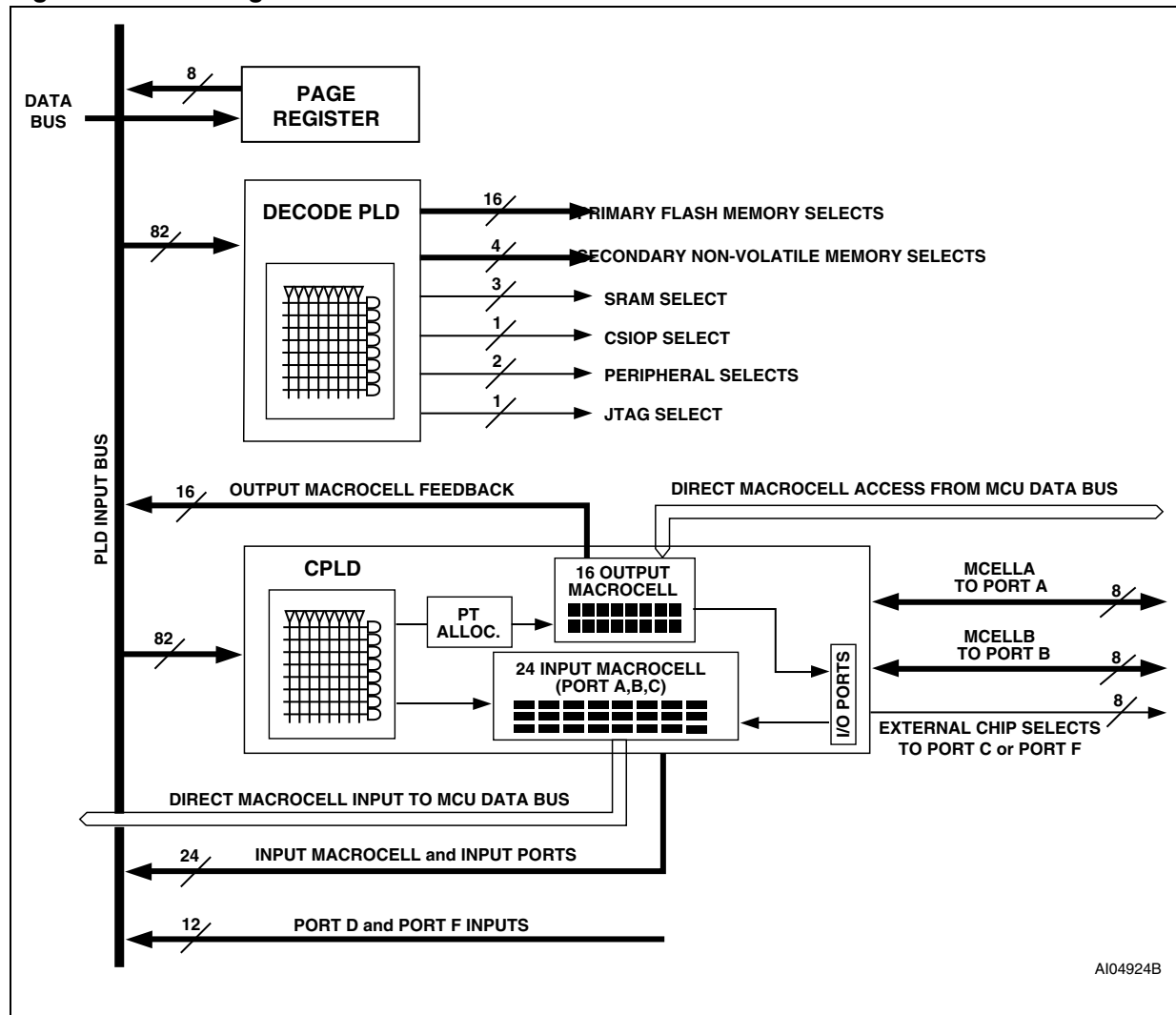
Figure 11. PLD diagram
