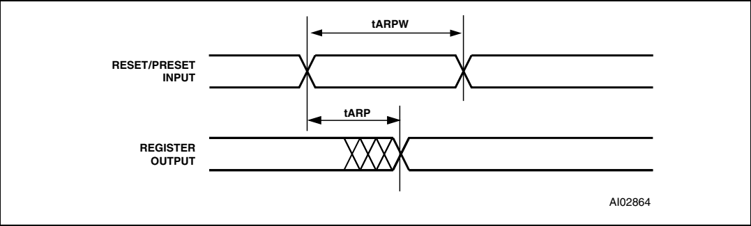
Figure 44. Asynchronous RESET / Preset
