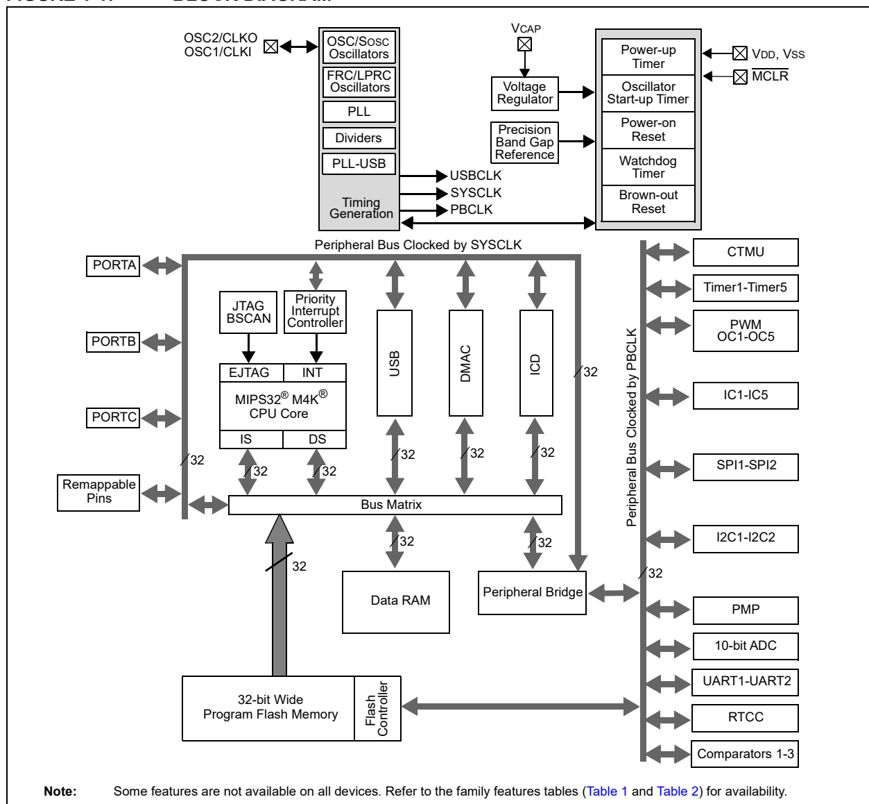
FIGURE 1-1: BLOCK DIAGRAM
