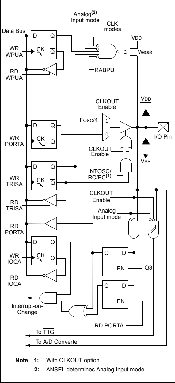
FIGURE 6-5: BLOCK DIAGRAM OF RA4
