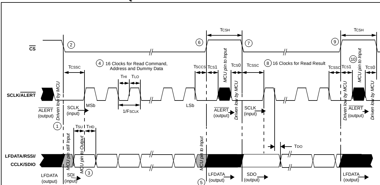
FIGURE 11-18: SPI READ SEQUENCE
