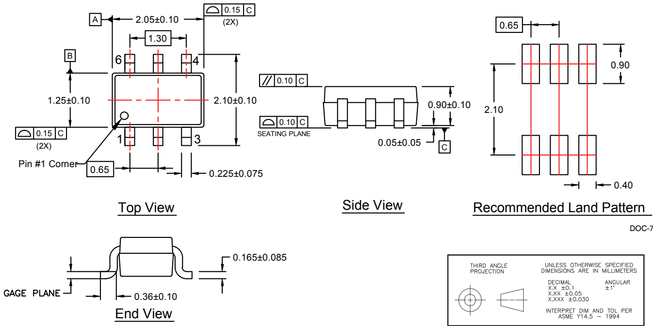
Figure 15. Package Drawing 6-lead SC-70
