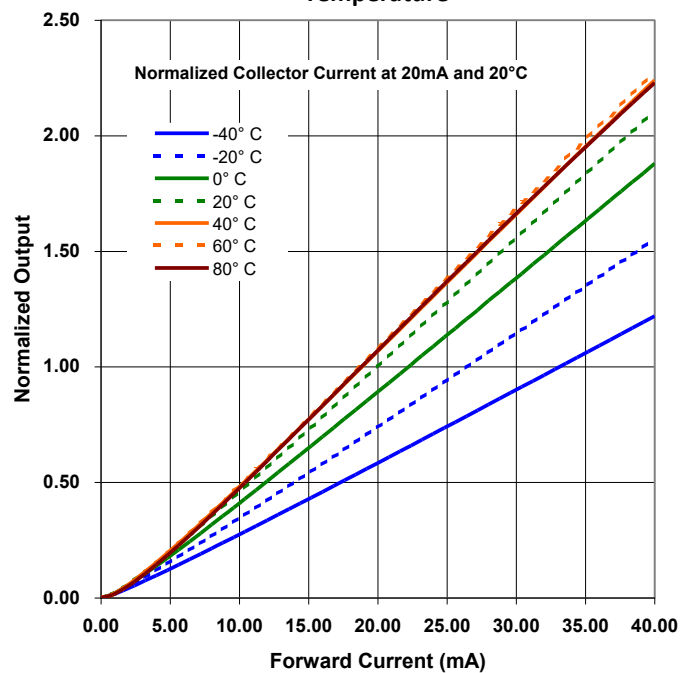
Darlington Output vs Forward Current vs Temperature
