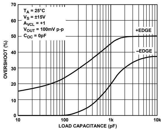
Figure 22. Small Signal Overshoot vs. Capacitive Load
