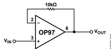
Figure 33. Unity-Gain Follower
