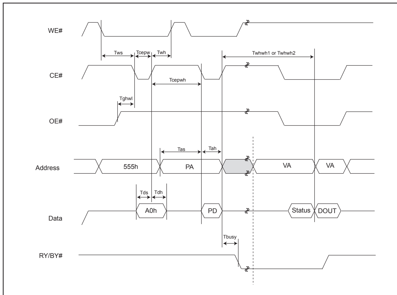
Figure 14. CE# CONTROLLED WRITE TIMING WAVEFORM
