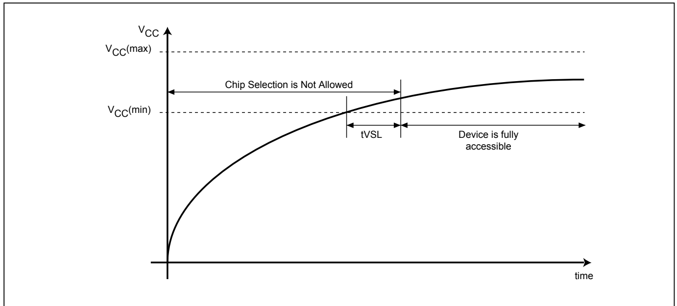
Figure 33. Power-up Timing
