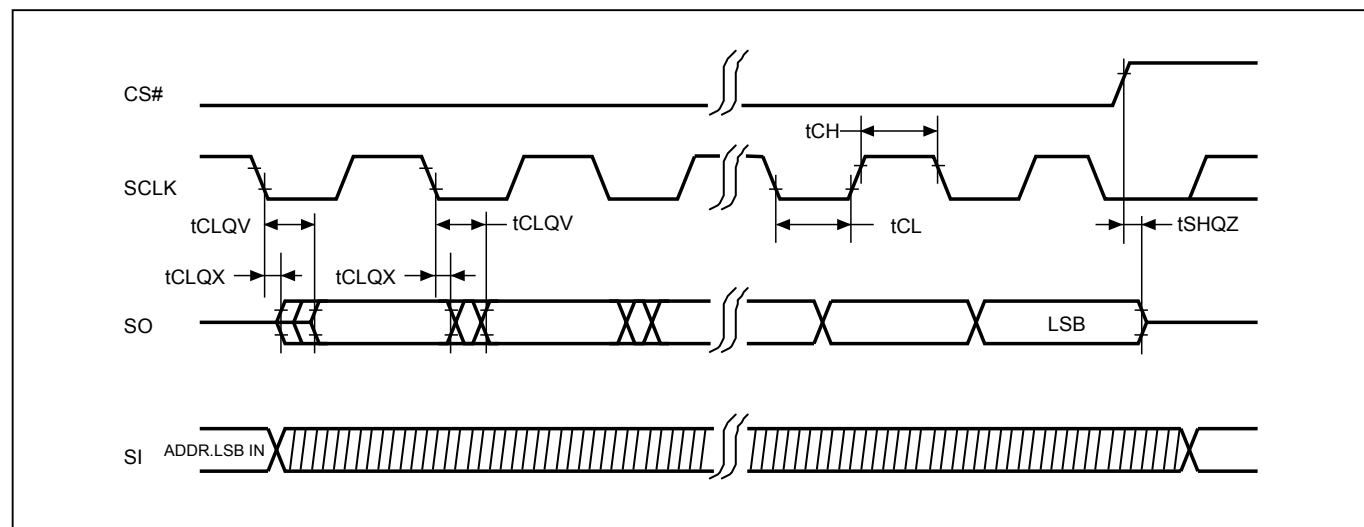
Figure 9. Output Timing
