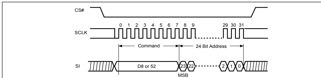
Figure 21. Block Erase (BE) Sequence (Command D8 or 52)
