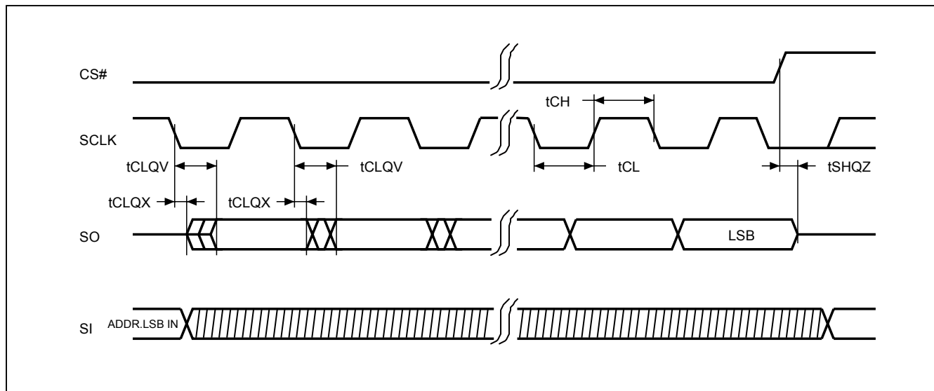
Figure 41. Output Timing
