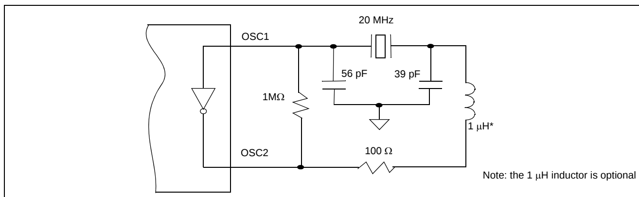
Figure 9 - Crystal Oscillator Circuit
