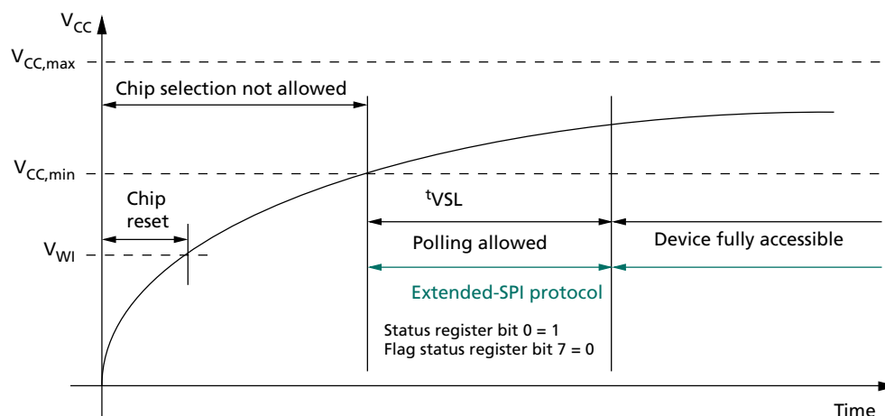
Figure 45: Power-Up Timing
