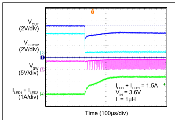
FIGURE 2-22: Overvoltage Protection Recovery.
