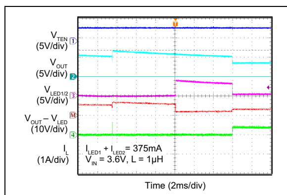
FIGURE 2-20: LED Open-Circuit Protection Recovery.
