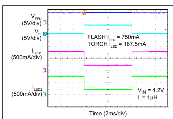
FIGURE 2-23: Flash Inhibit and Recovery.
