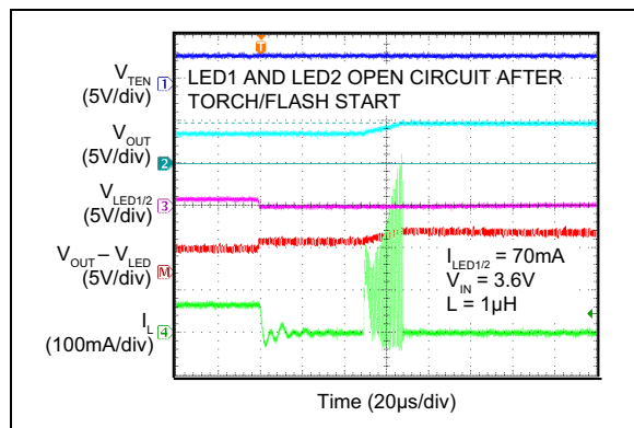
FIGURE 2-19: LED Open-Circuit Protection.
