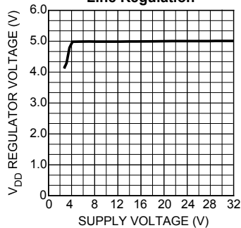
V_{DD} Line Regulation
