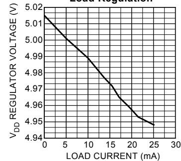
V_{DD} Load Regulation
