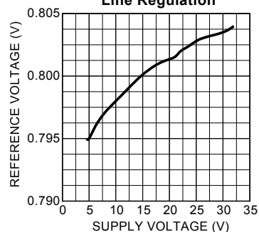
V_{FB} Line Regulation
