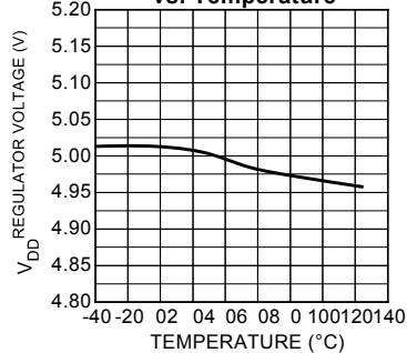
V_{DD} vs. Temperature
