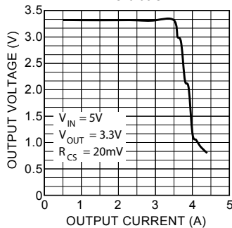
Current Limit Foldback
