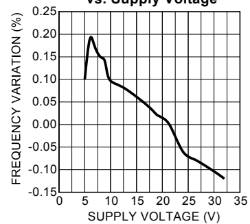
Oscillator Frequency vs. Supply Voltage
