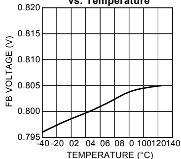
V_{FB} vs. Temperature
