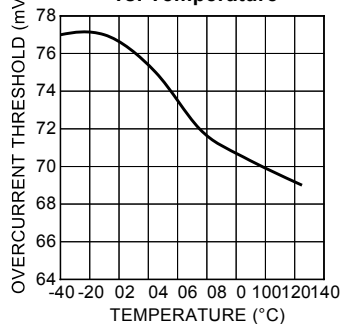
Overcurrent Threshold vs. Temperature
