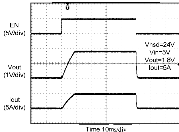
Power-Up/Power-Down
