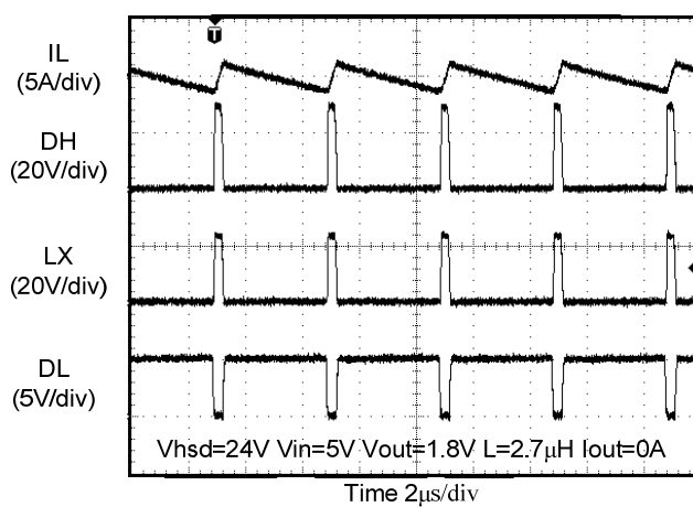
Switching Waveform (No Load)
